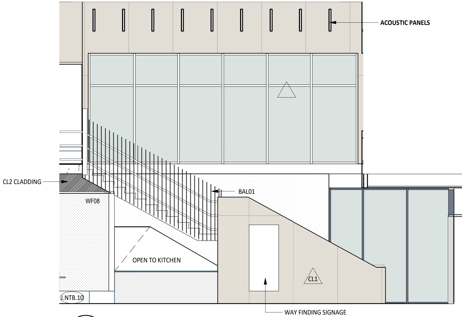
5 ELEVATION DETAIL 1 : 50
