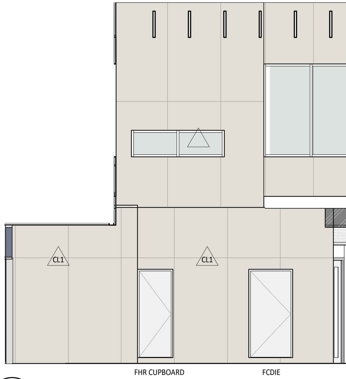
3 ELEVATION DETAIL 1 : 50
