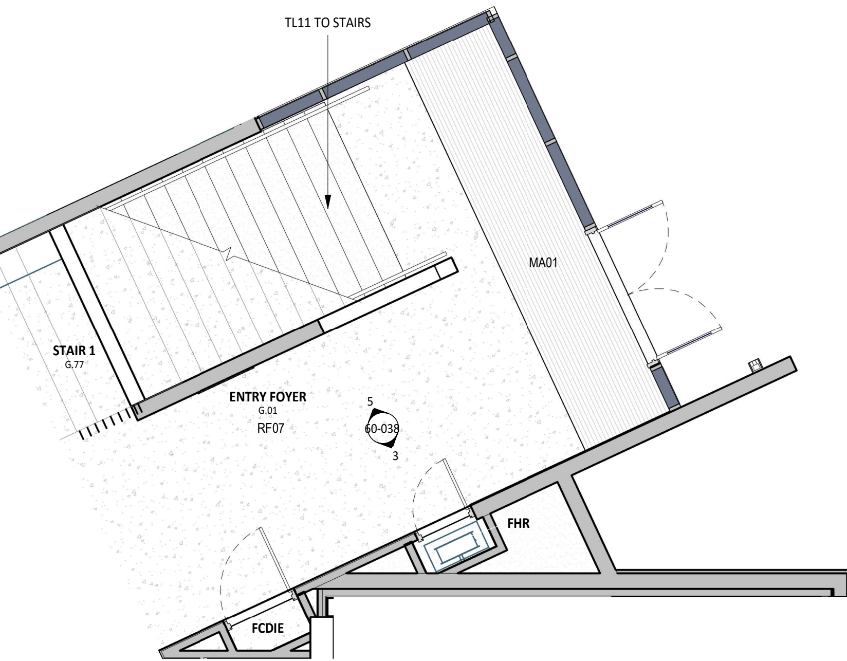
1 PLAN DETAIL - GROUND LEVEL 1 : 50
